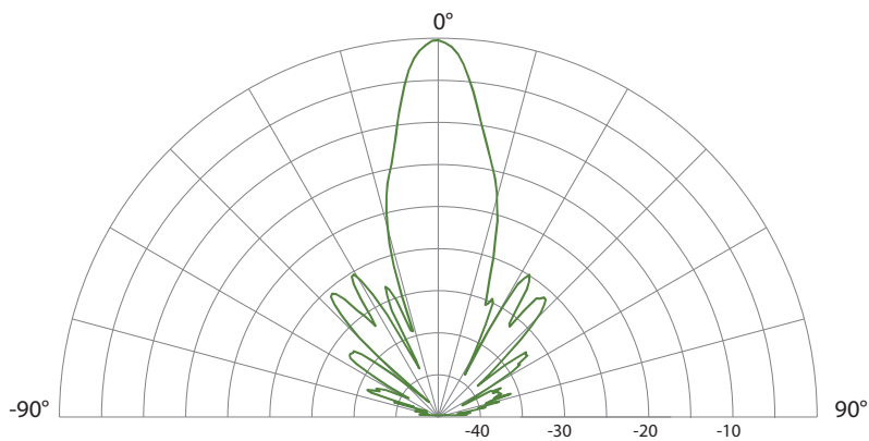
Azimuth (measured @61GHz)
