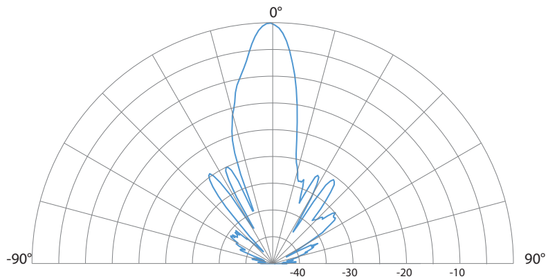
Elevation (measured @61GHz)
